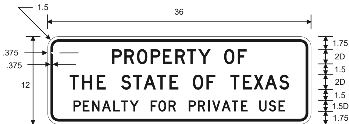
TX3-1T PROPERTY OF THE STATE OF TEXAS PENALTY FOR PRIVATE USE
