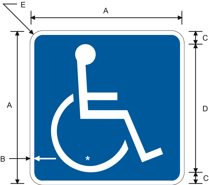
D9-6 Handicapped (Symbol)
