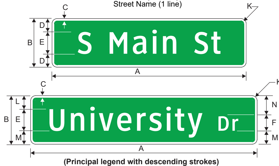
D3-1G (Green) Street Name (1 line)
