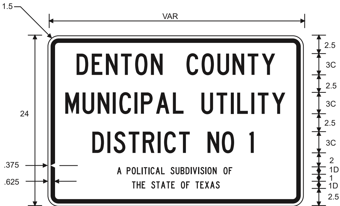
TX5-2T COUNTY MUNICIPAL UTILITY DISTRICT NO
