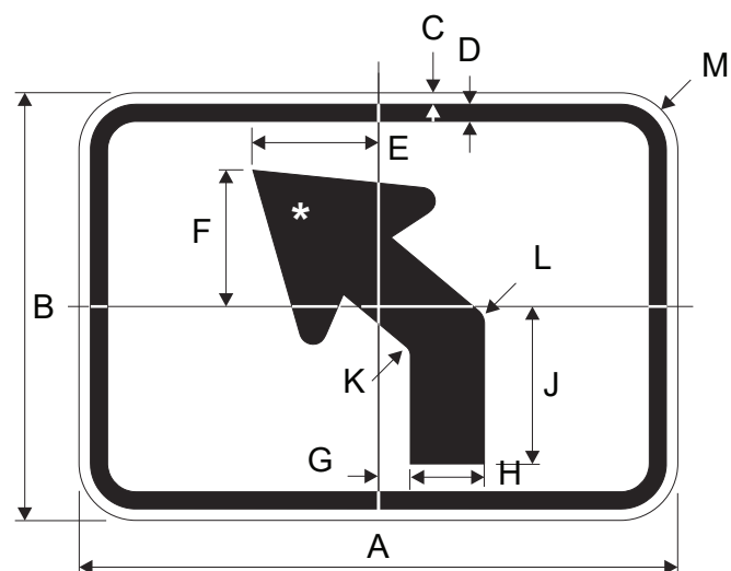
M5-2L (R)
