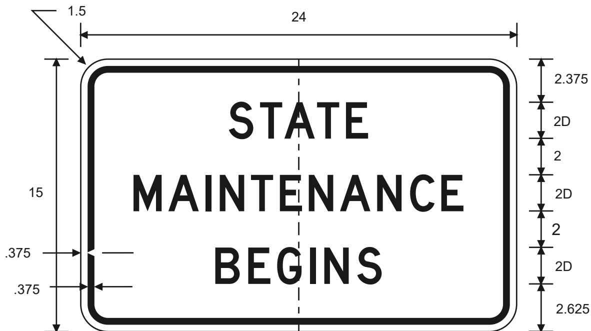
TX1-2T STATE MAINTENANCE BEGINS
