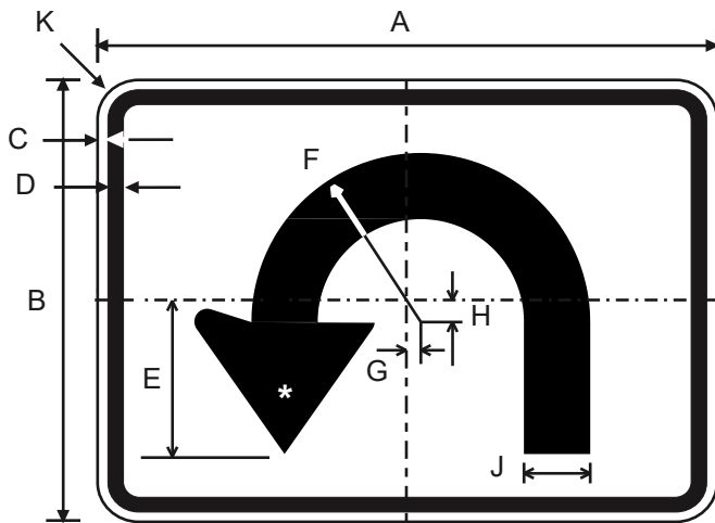
Advance Turn Arrow Circular Intersection
