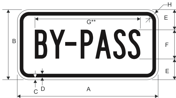
M4-2 BY-PASS
