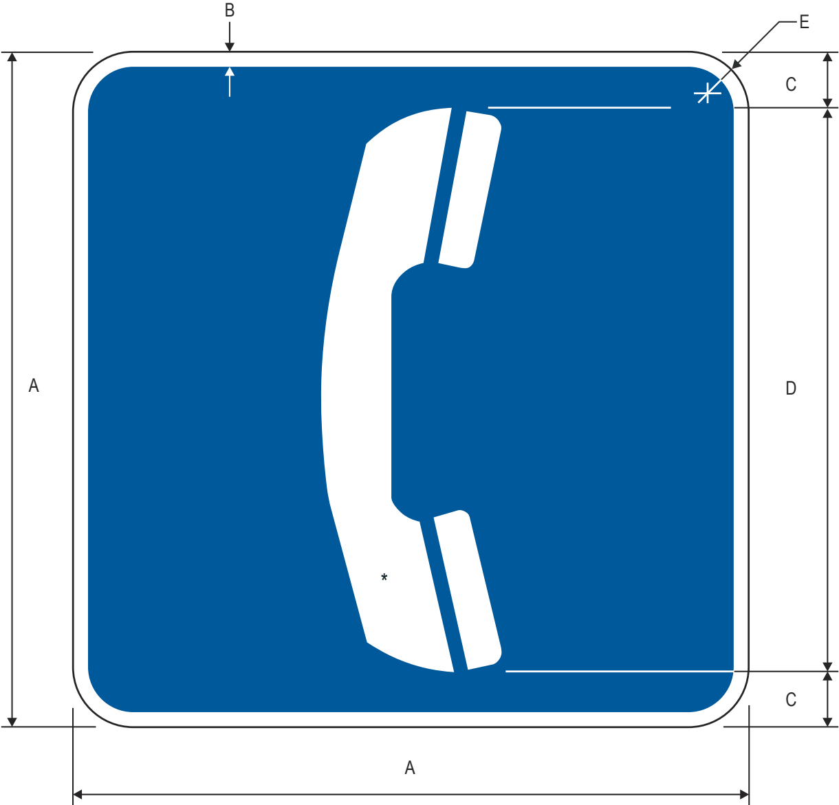
D9-1 Phone (Symbol)
