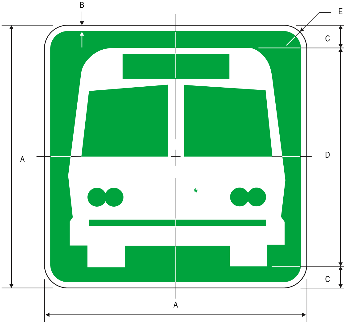
I-6 Bus Station (Symbol)
