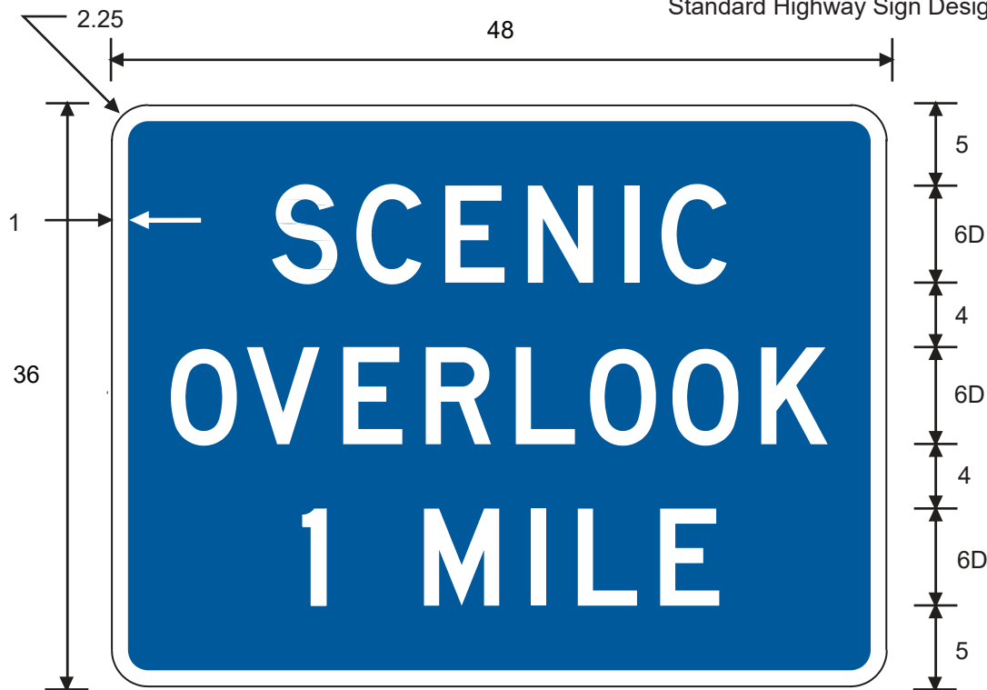
D5-1eT SCENIC OVERLOOK X MILE
