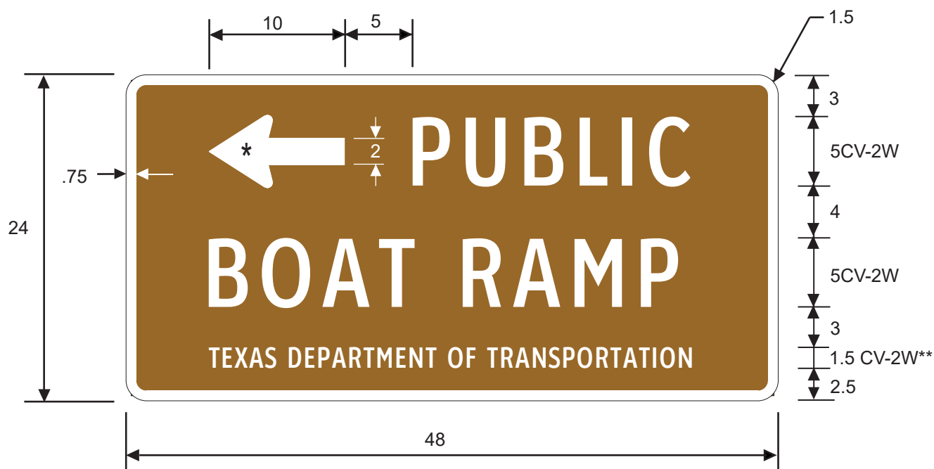
D7-5TL
