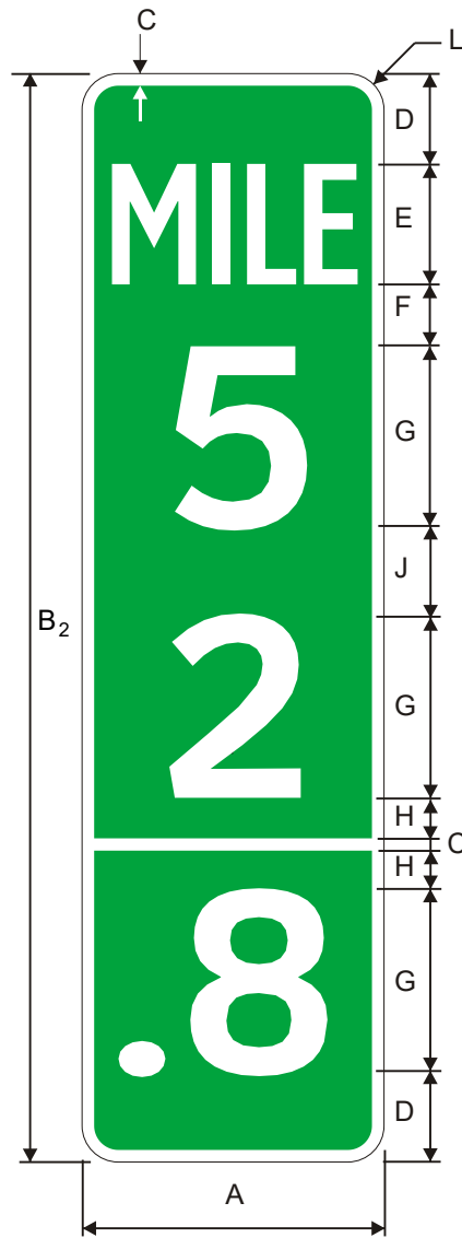
D10-2a Texas Number Reference Location (2 number with decimal)
