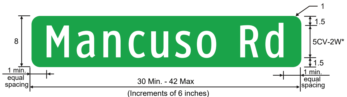
D3-4aT COUNTY ROAD NAME
