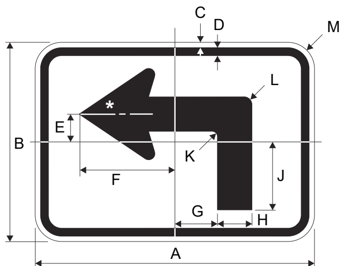
M5-1L (R)
