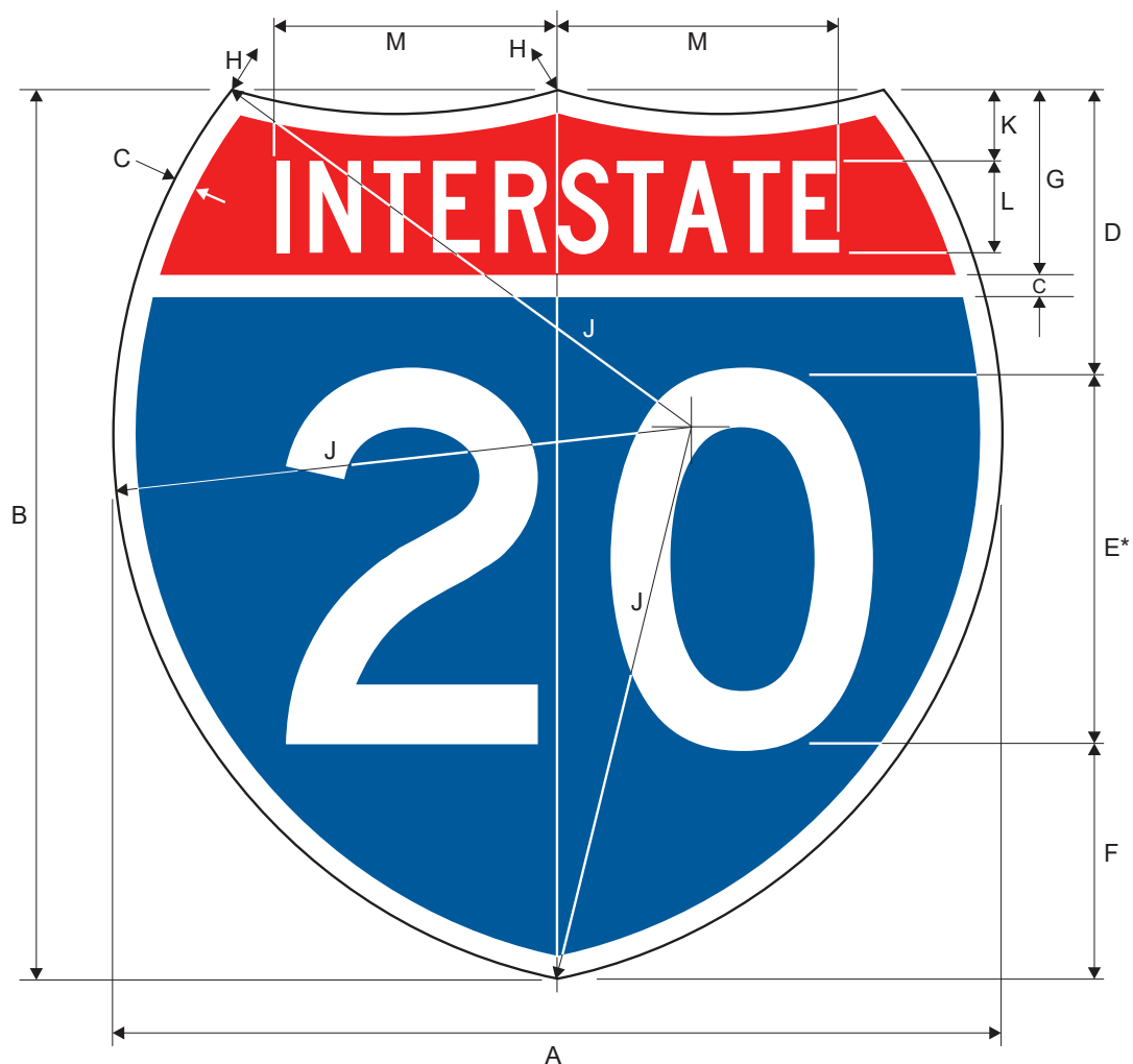
M1-1 Interstate Route Markers (Attachment)
