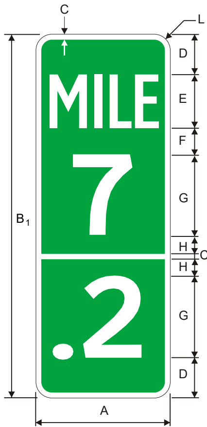
D10-1a Texas Number Reference Location (1 number with decimal)
