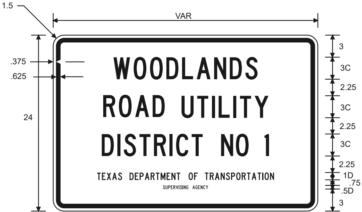
TX5-1T WOODLANDS ROAD UTILITY DISTRICT NO 1
