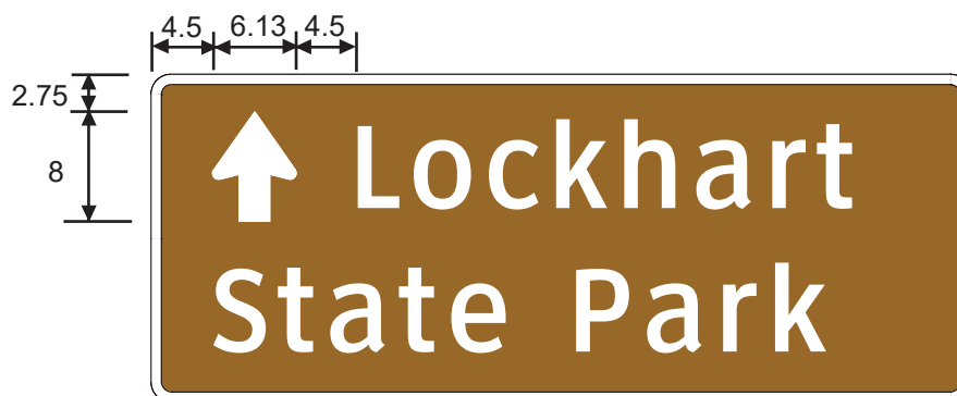
D7-1T (UP) STATE / NATIONAL PARK (Arrow)
