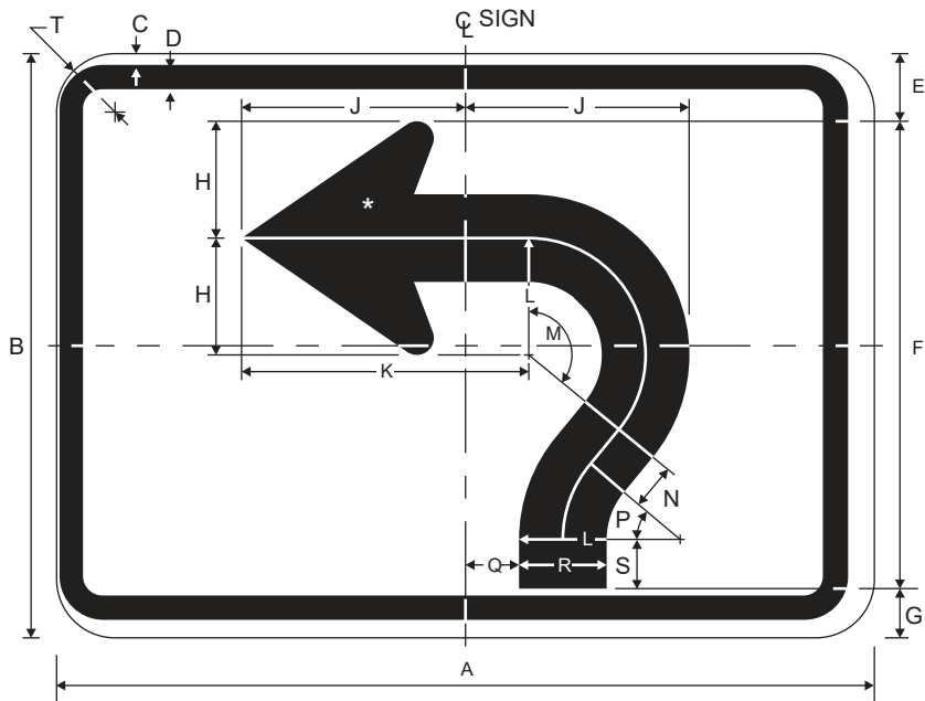
Advance Turn Arrow Circular Intersection
