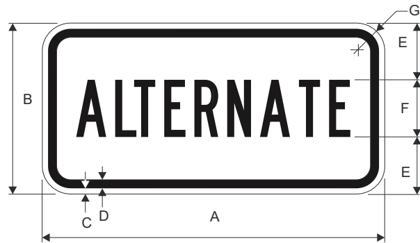
M4-1 ALTERNATE
