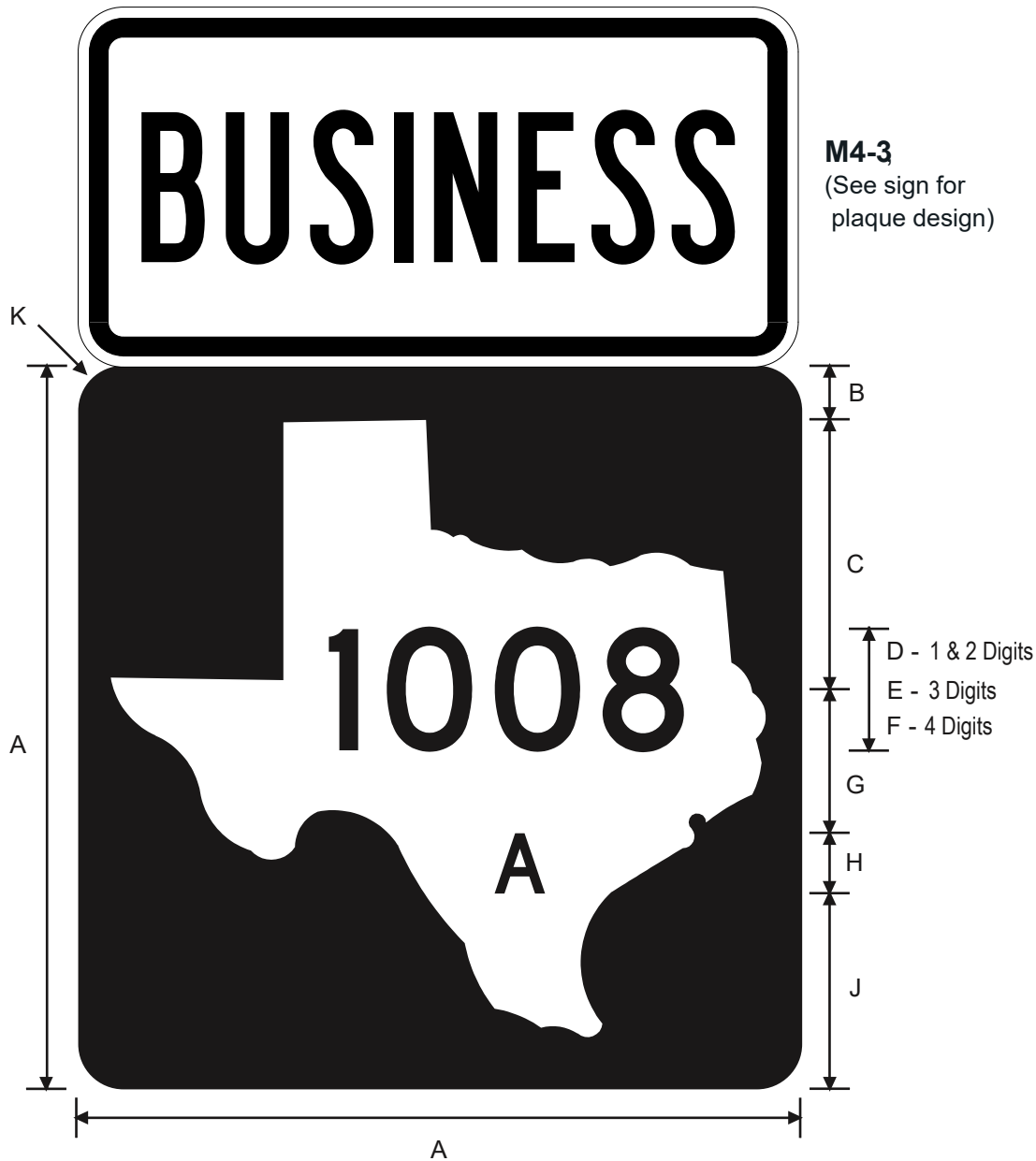
M1-6FB Texas Business Assembly Road Route Marker (Independent)
