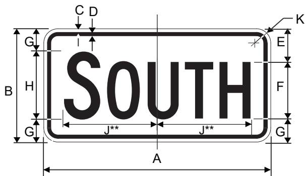
M3-3 SOUTH
