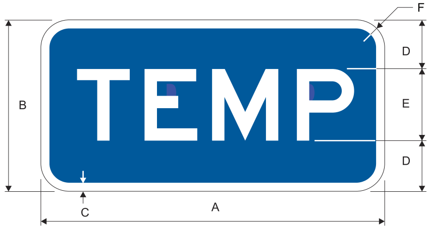
M4-7aB (Blue)
