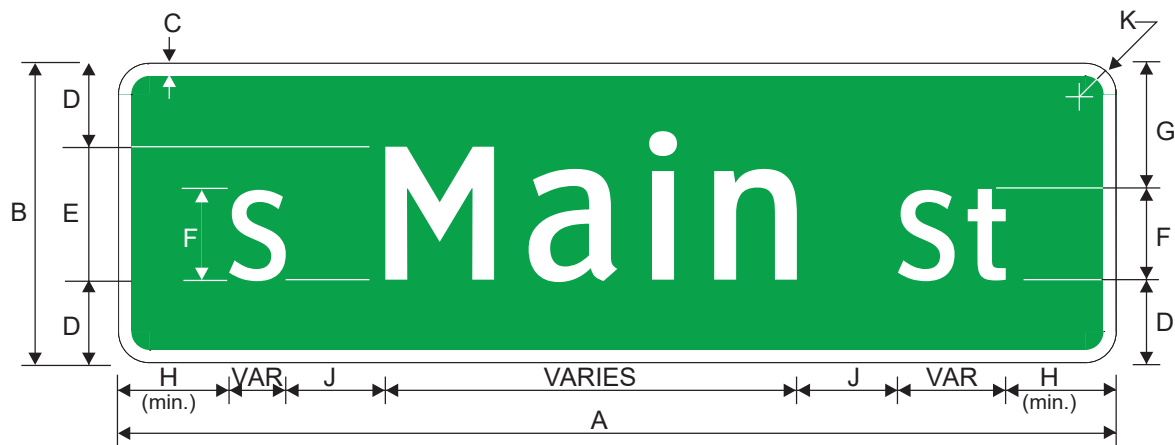
D3-1G (Green) Street Name (1 line)
