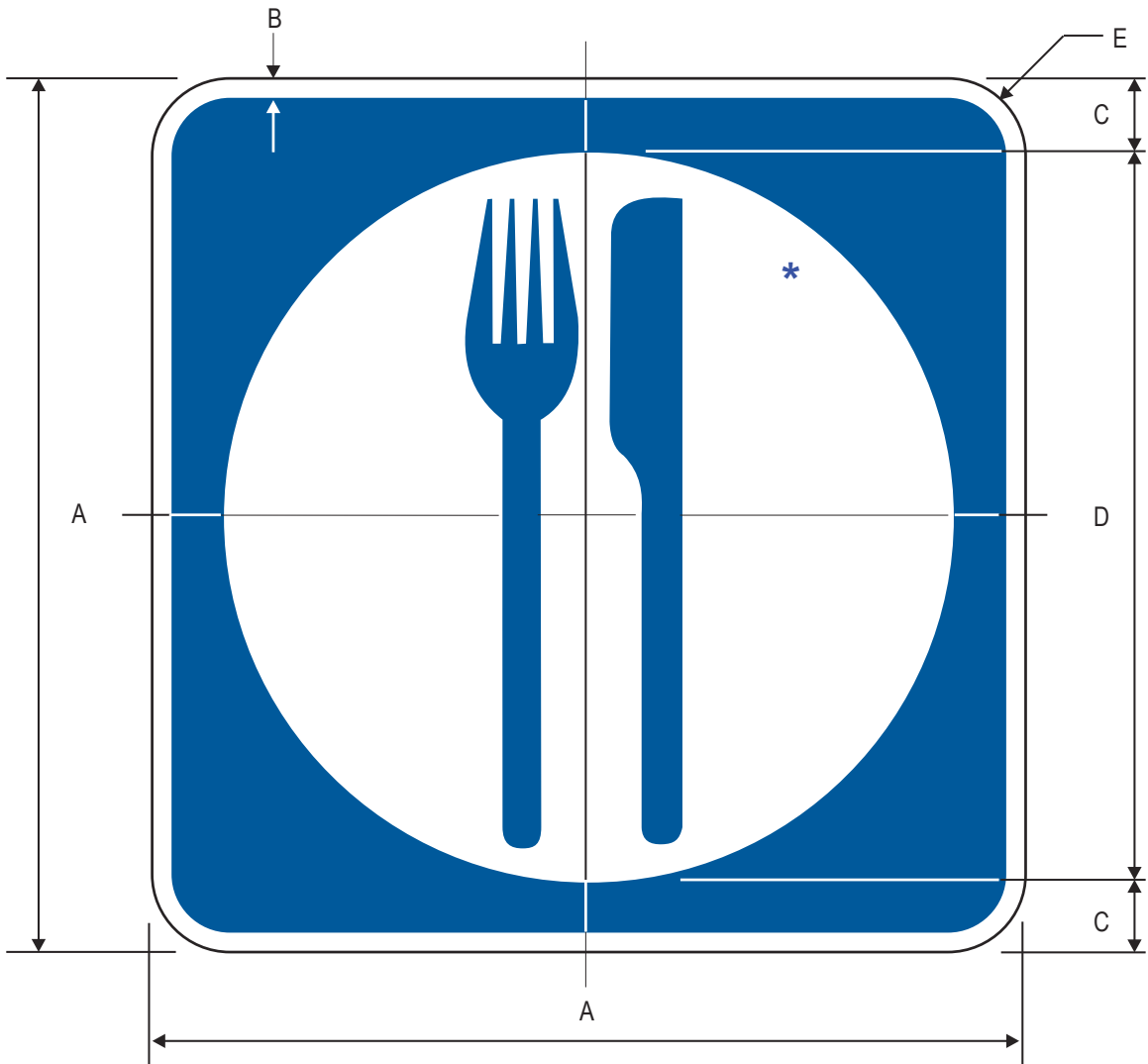
D9-8 Food (Symbol)
