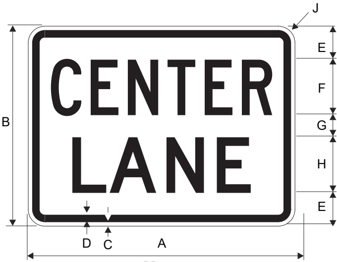
M5-5 CENTER LANE
