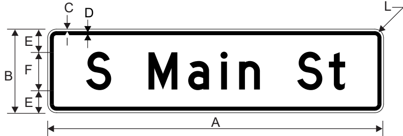
D3-1 Street Name (1 line)
