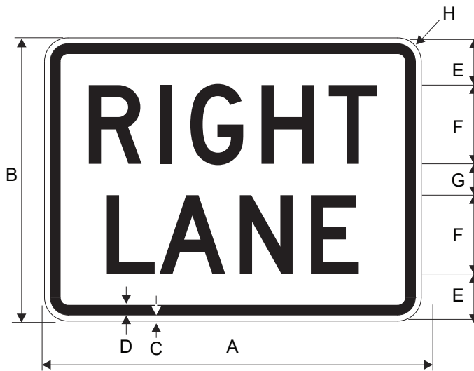
M5-6 RIGHT LANE
