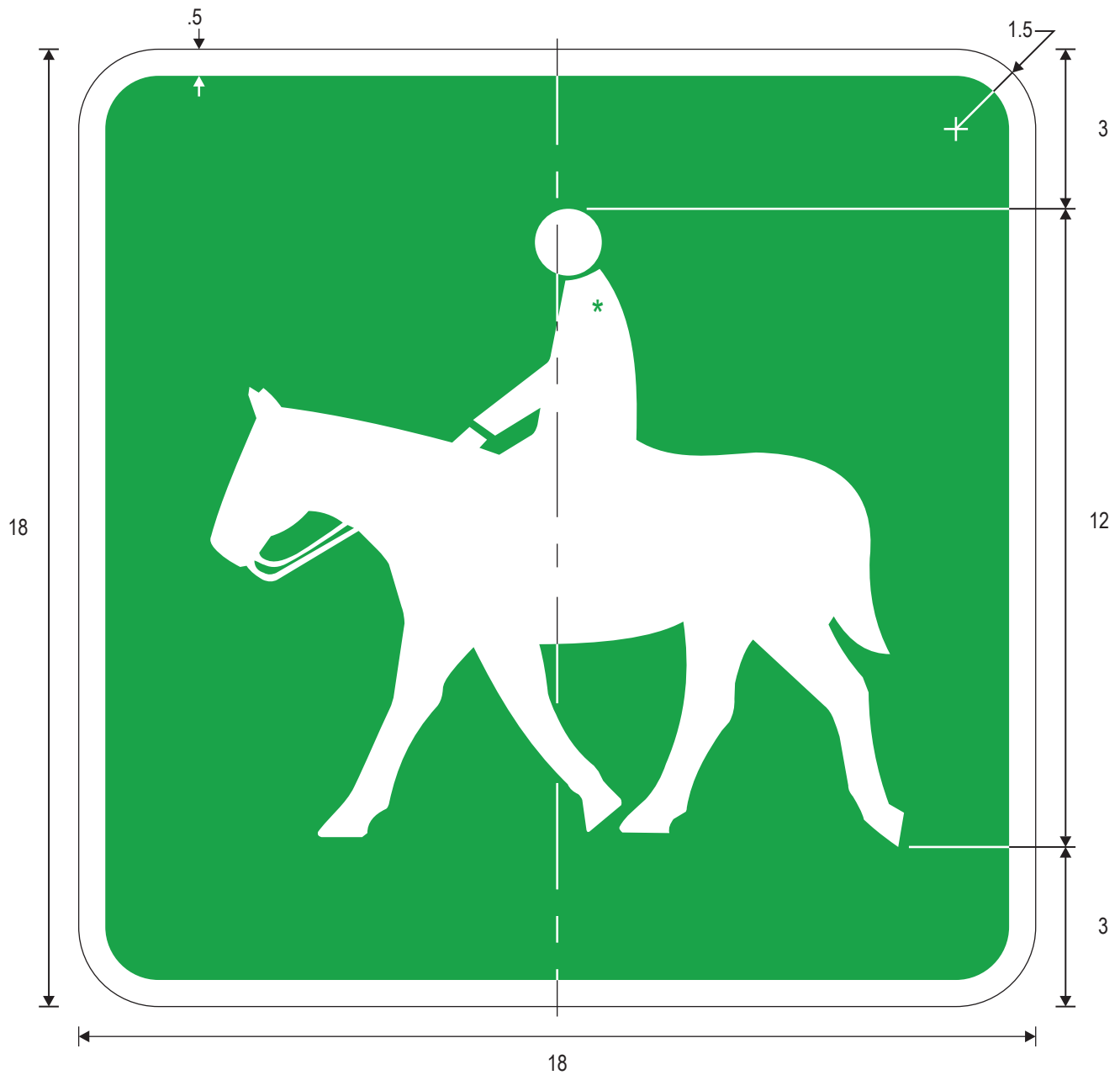
D11-4 Equestrians Permitted (Symbol)
