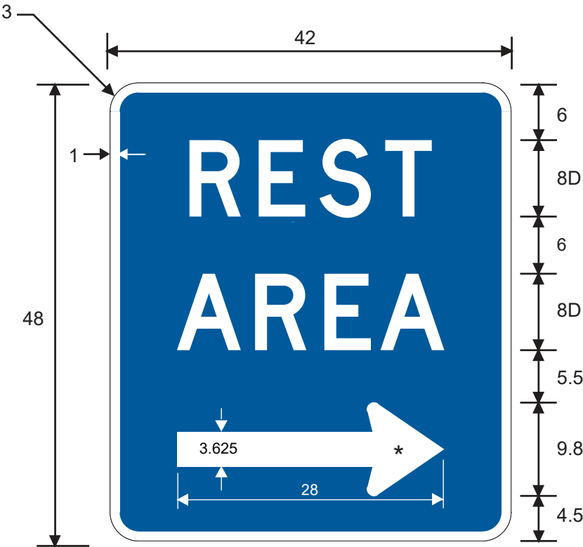
D5-5R REST AREA (with Arrow)
