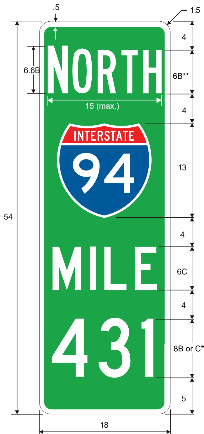
D10-4 Enhanced Reference Location (Number and shield)
