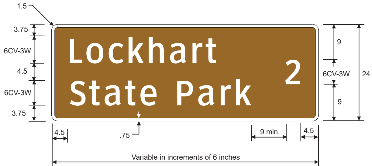
D7-2T Distance STATE PARK
