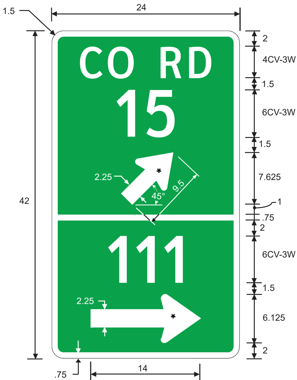
D20-9T (R45, R) COUNTY ROAD
