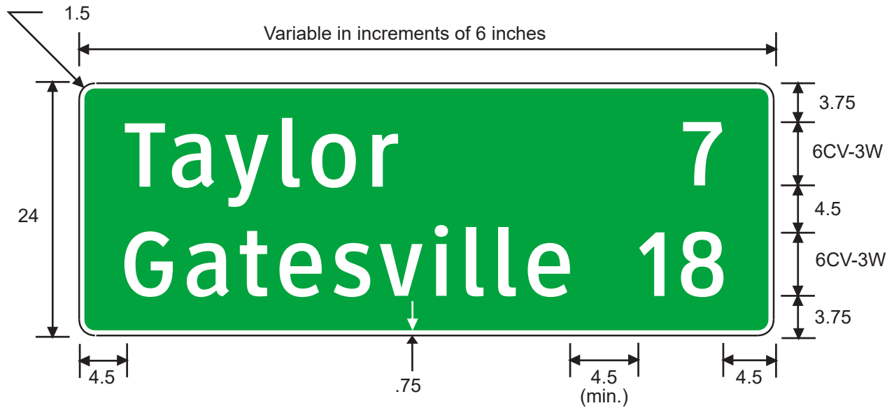
D2-2 Distance (2 line)
