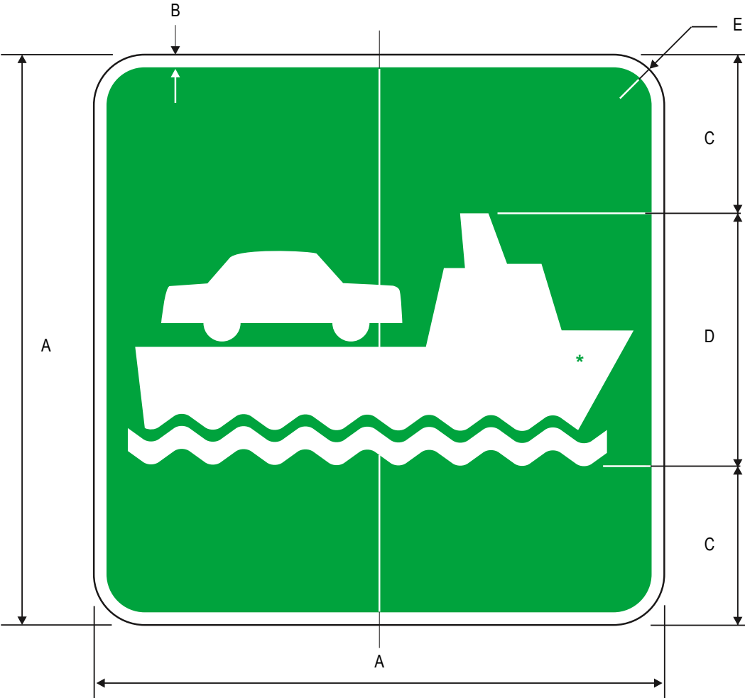
I-9 Vehicle Ferry Terminal (Symbol)
