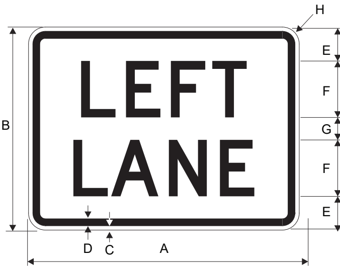
M5-4 LEFT LANE
