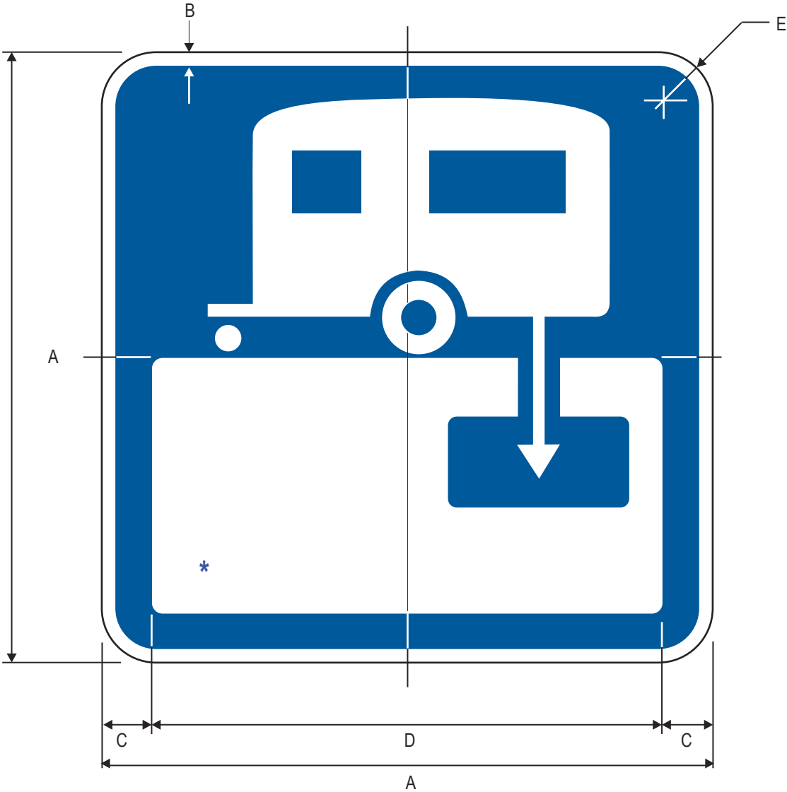
D9-12 RV Sanitary Station (Symbol)
