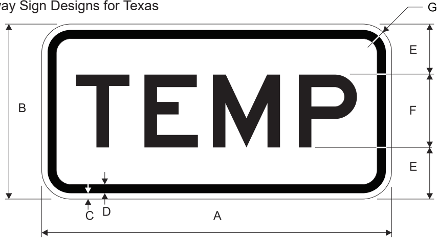
M4-7a TEMP
