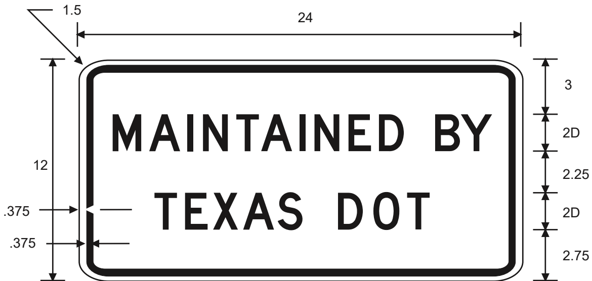
TX1-4T MAINTAINED BY TEXAS DOT
