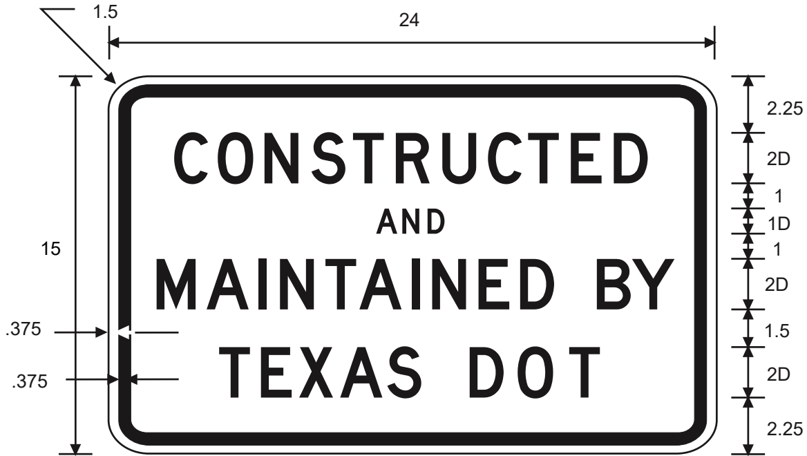
TX1-3T CONSTRUCTED AND MAINTAINED BY TEXAS DOT
