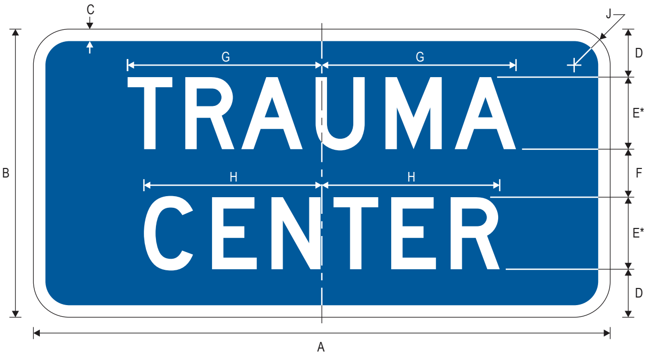
D9-13dP TRAUMA CENTER (Plaque)
