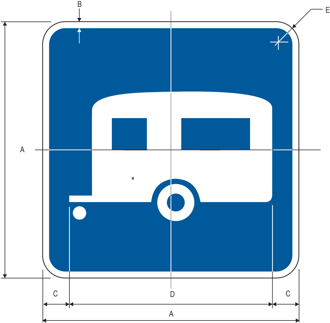
D9-3a Trailer Camping (Plaque)
