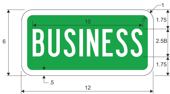
M4-3G* BUSINESS
