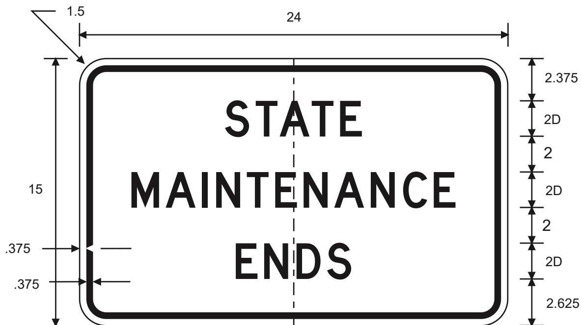
TX1-1T STATE MAINTENANCE ENDS
