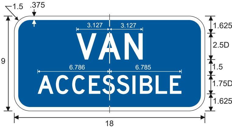
D9-6P VAN ACCESSIBLE (Plaque) COLORS: LEGEND - WHITE BACKGROUND - BLUE
