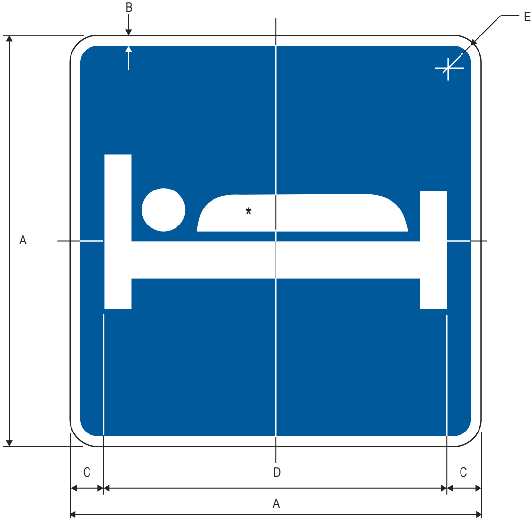
D9-9 Lodging (Symbol)
