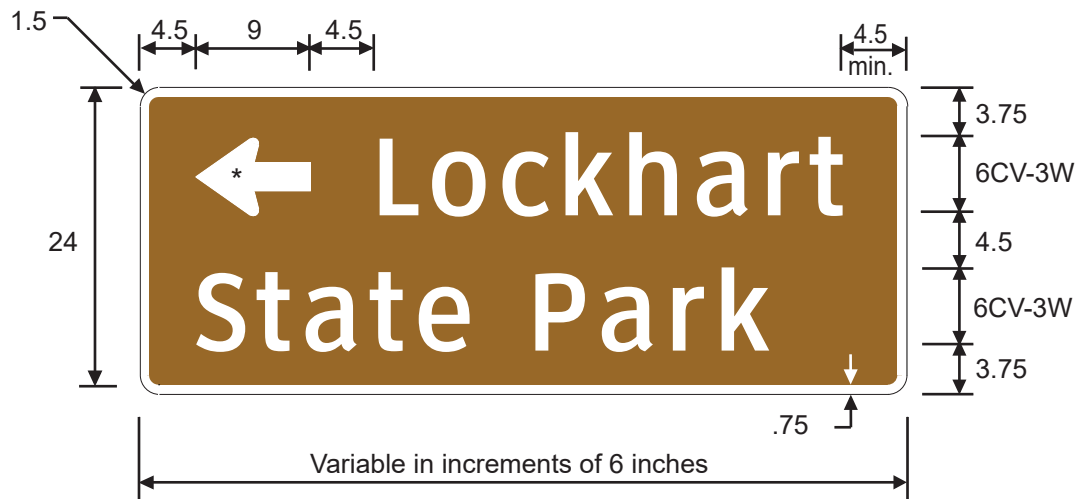
D7-1T (L) STATE / NATIONAL PARK (Arrow)
