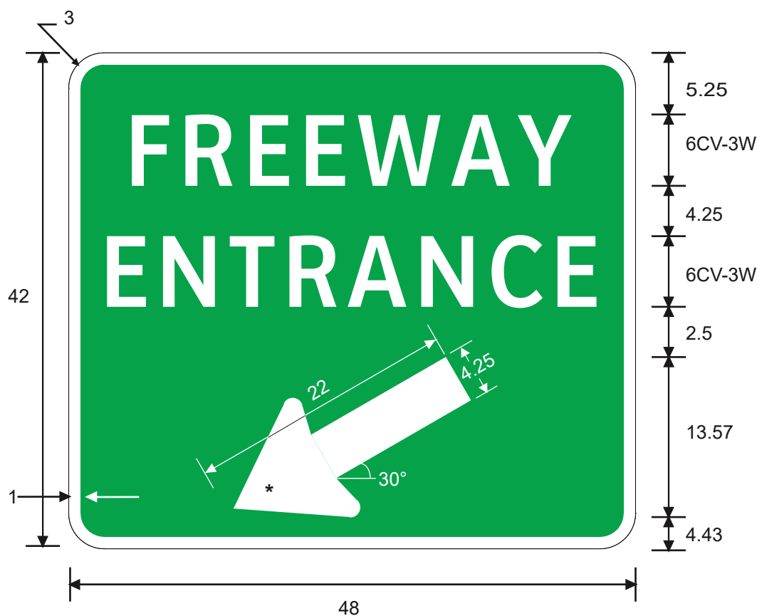
D13-3a FREEWAY ENTRANCE (30 Degree arrow)
