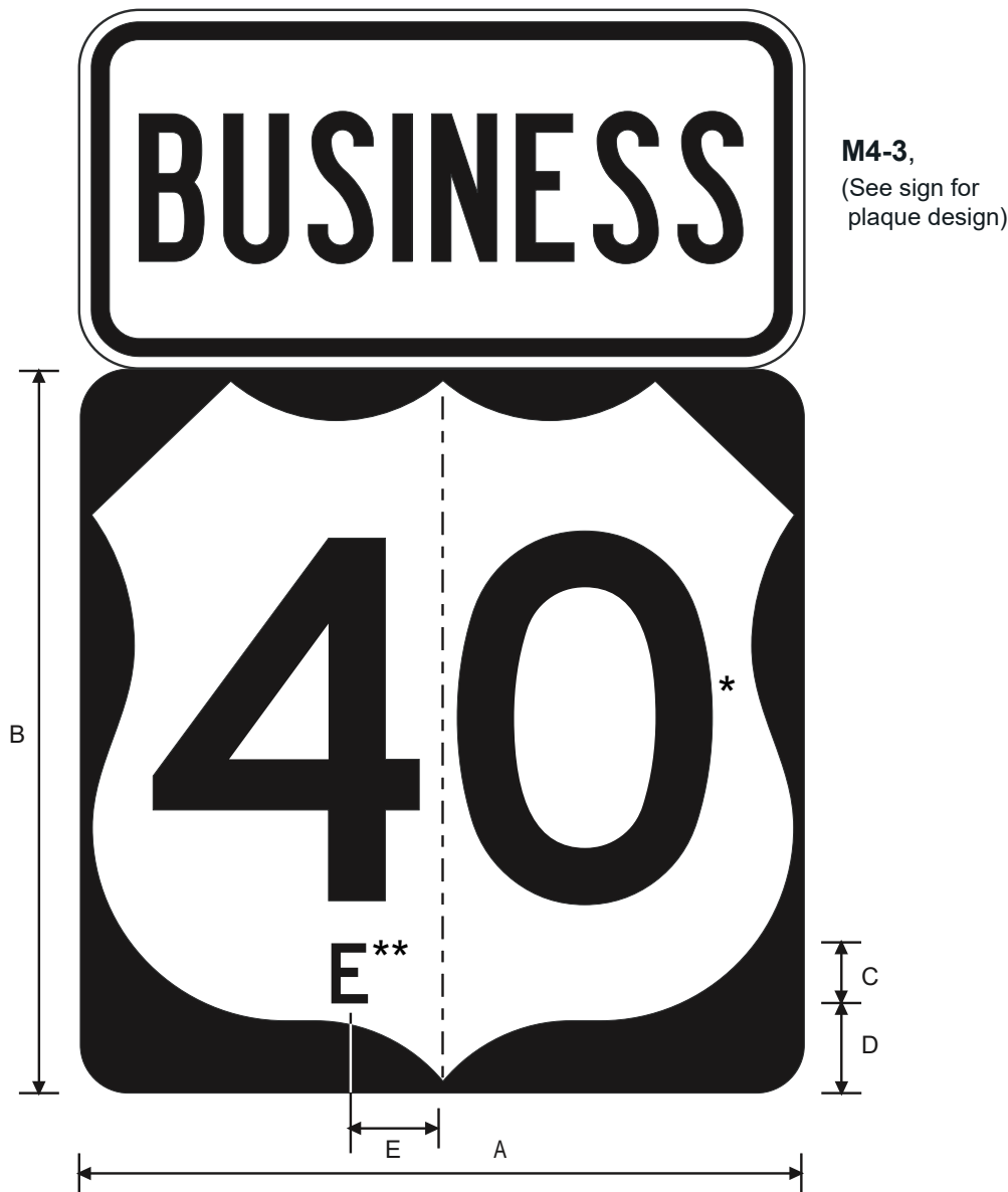
M1-4B U.S. Business Route Marker Assembly (Independent)
