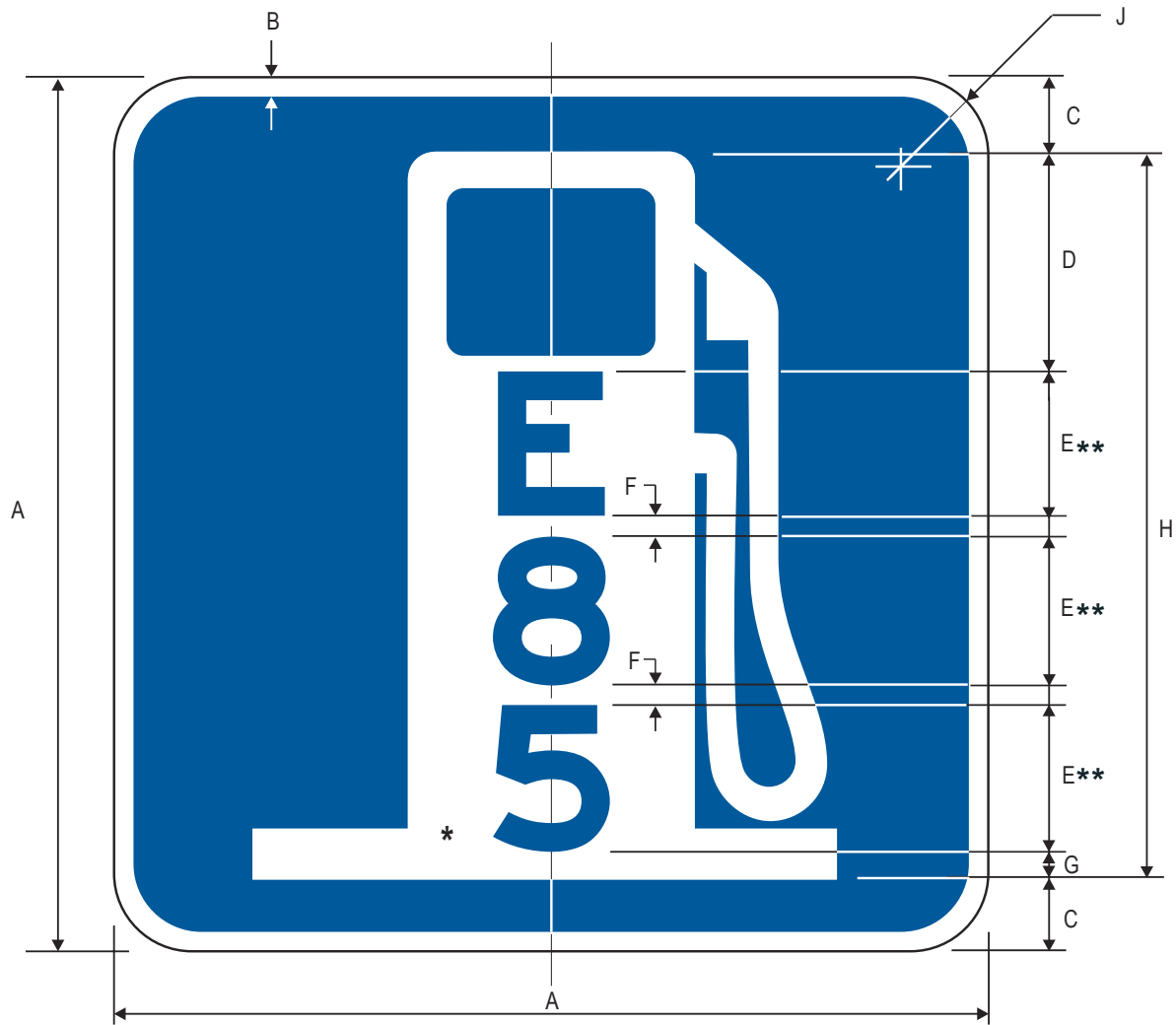
D9-11c Gas E85 (Symbol)
