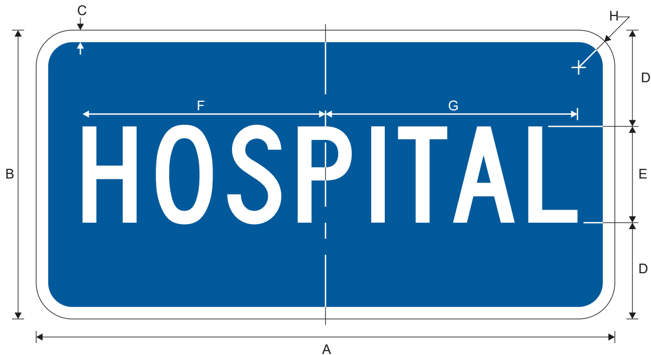
D9-13aP HOSPITAL (Plaque)
