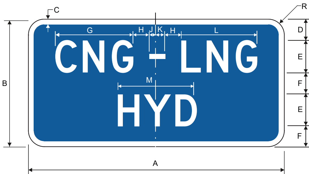
D9-11gPT
