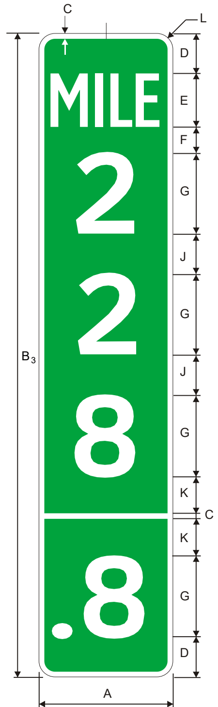
D10-3a Texas Number Reference Location (3 number with decimal)
