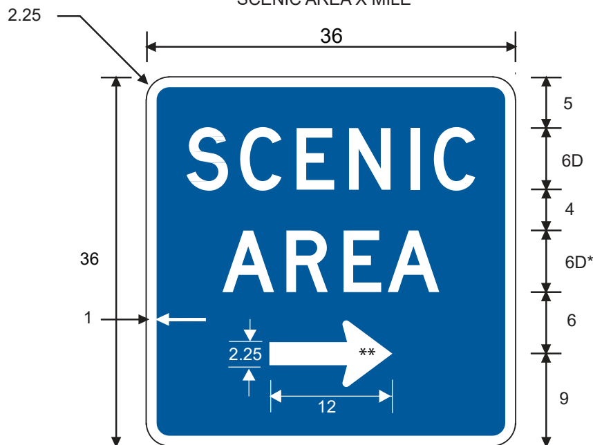
D5-2dTR SCENIC AREA (VIEW) (Arrow)
