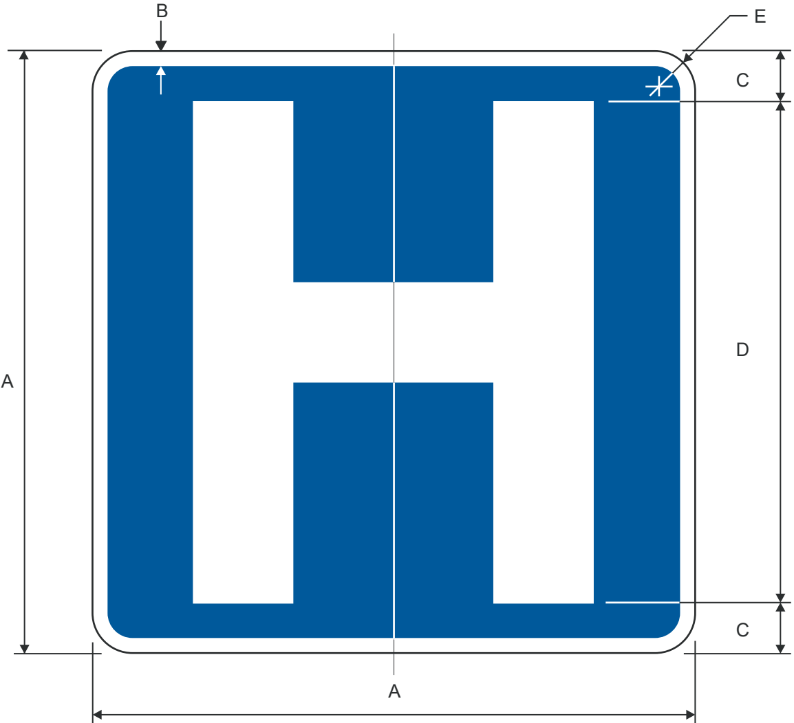
D9-2 Hospital (Plaque)
