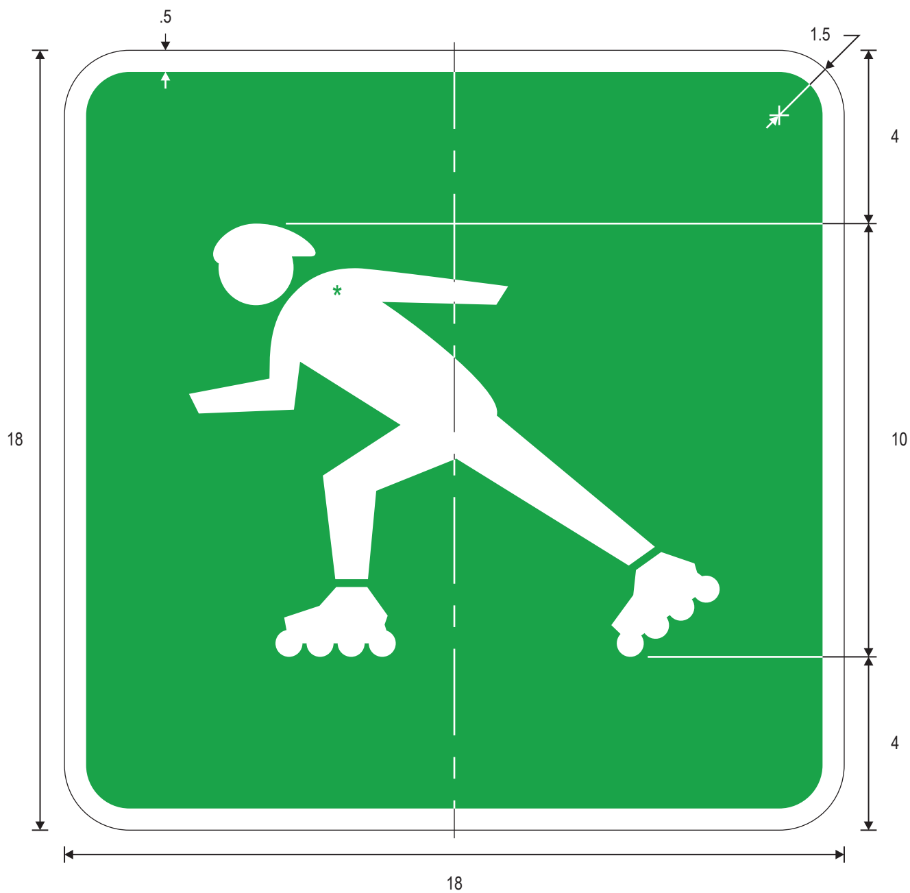
D11-3 Skaters Permitted (Symbol)
