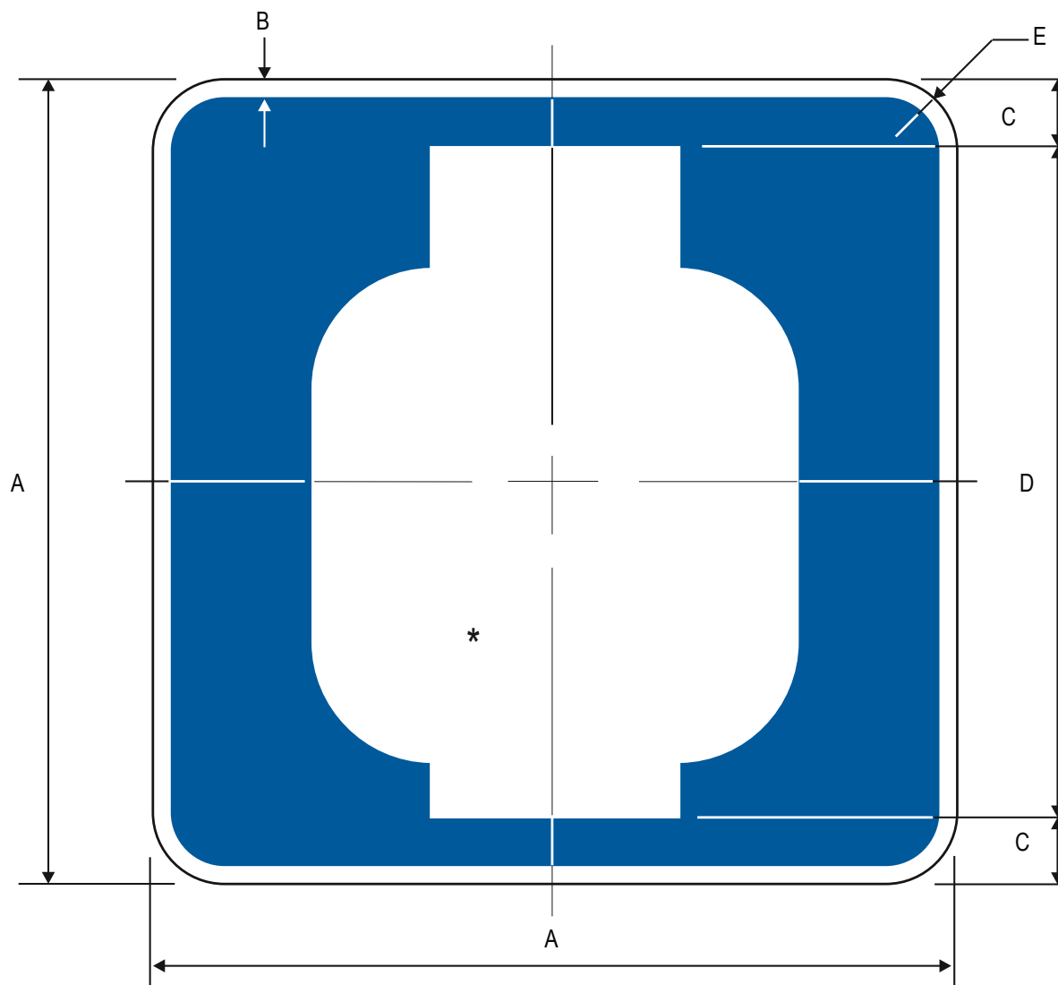
D9-15 Propane (Symbol)
