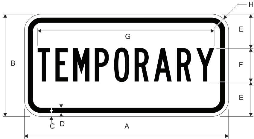
M4-7 TEMPORARY
