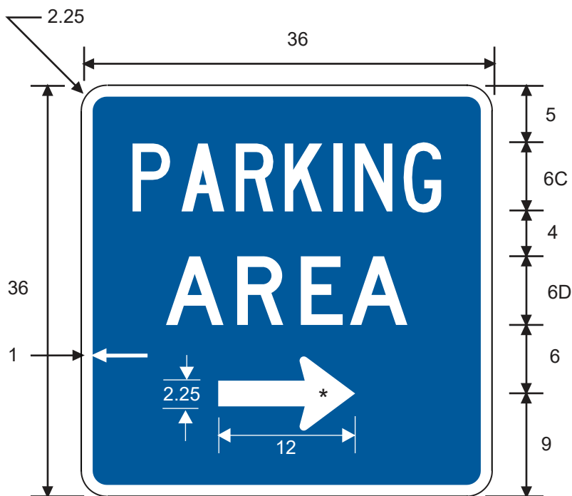
D5-2cTR PARKING AREA (Arrow)
