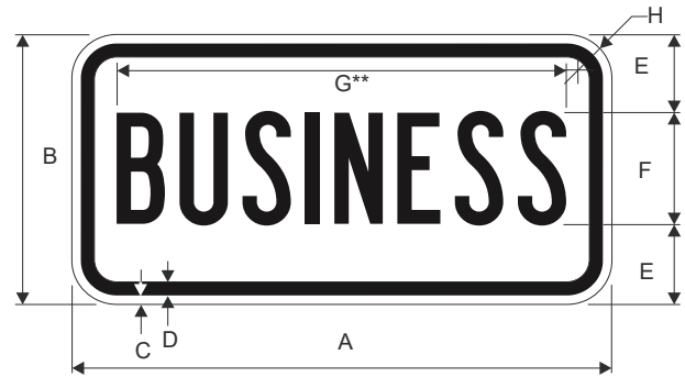
M4-3 BUSINESS
