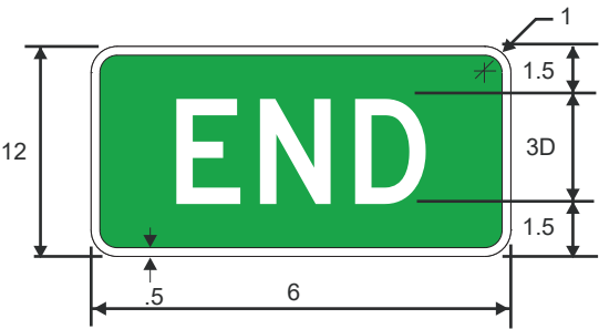
M4-6G* * For bicycle use
