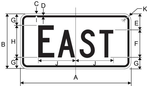
M3-2 EAST
