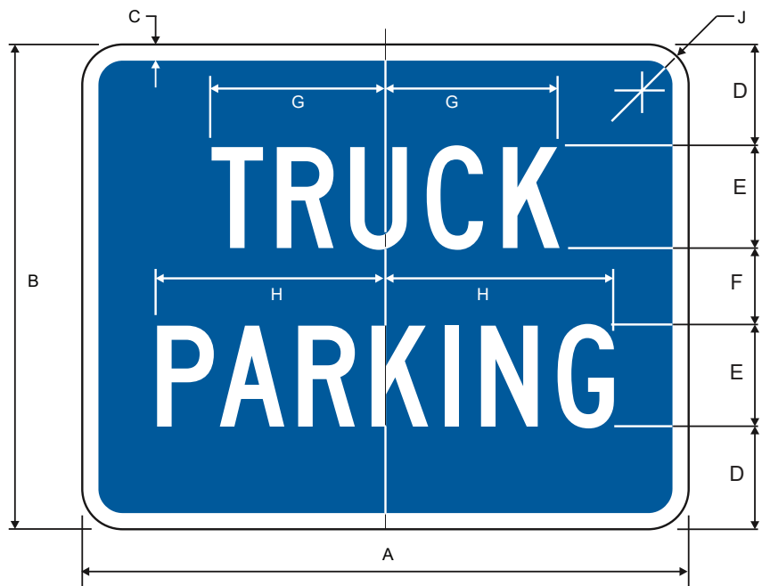
D9-16T TRUCK PARKING
