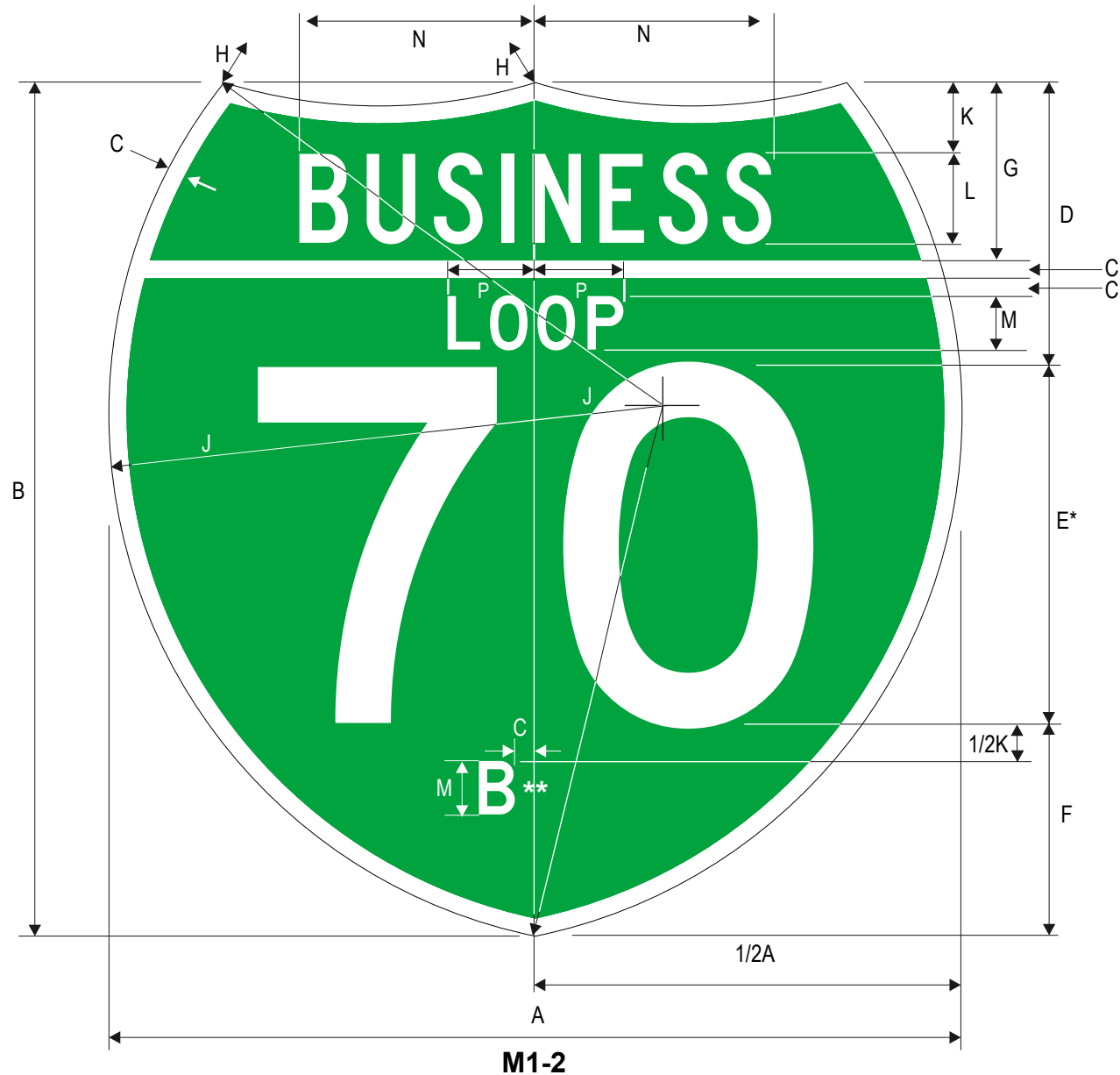
M1-2 Off Interstate Business Loop Marker (Attachment and Independent)
