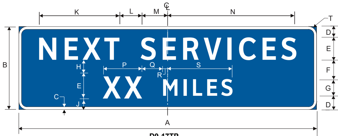
D9-17TP NEXT SERVICES XX MILES (Plaque)
