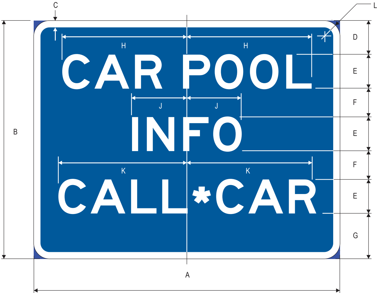
D12-2 CAR POOL INFO CALL * CAR
