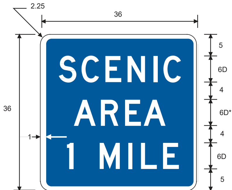
D5-1dT SCENIC AREA X MILE
