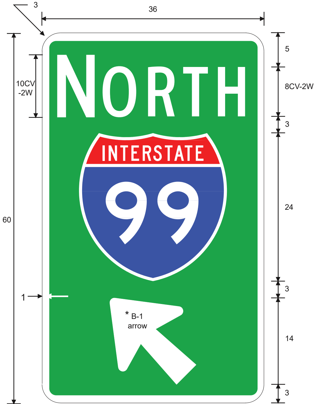
D13-4T FREEWAY ENTRANCE (45 Degree arrow and shield)
