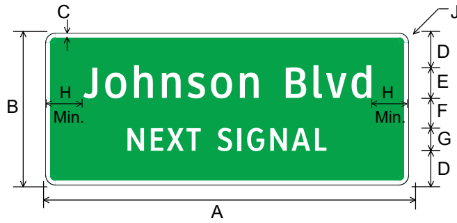
D3-2 (2 Lines)
