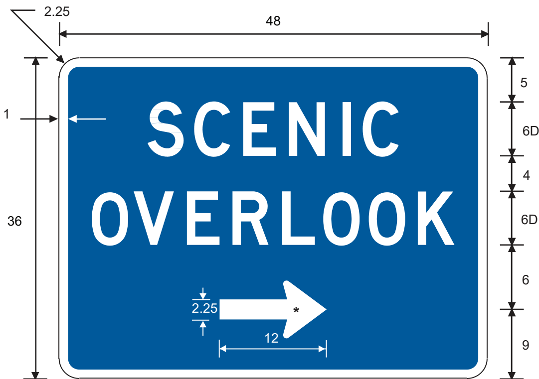
D5-2eTR SCENIC OVERLOOK (Arrow)
