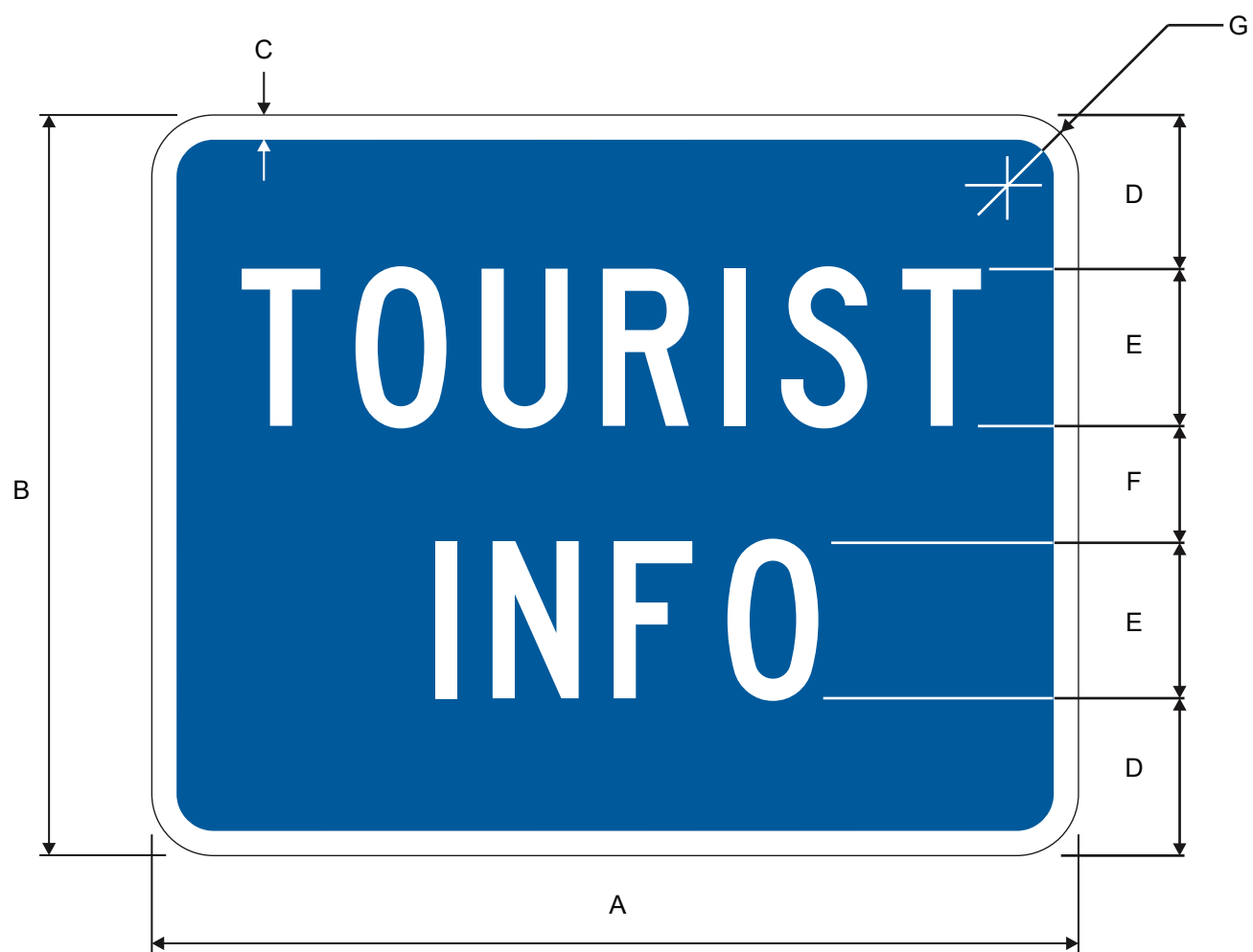
D9-10T TOURIST INFO
