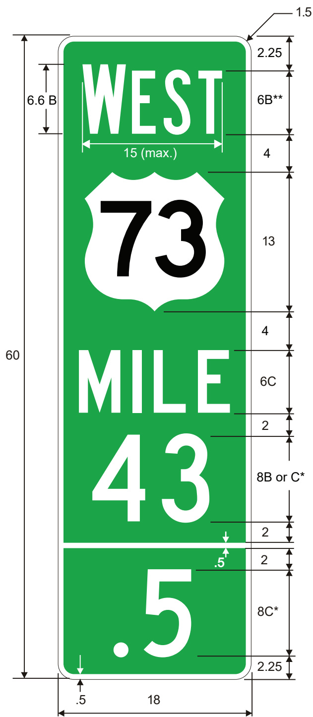
D10-5 Enhanced Reference Location (Number, decimal and shield)
