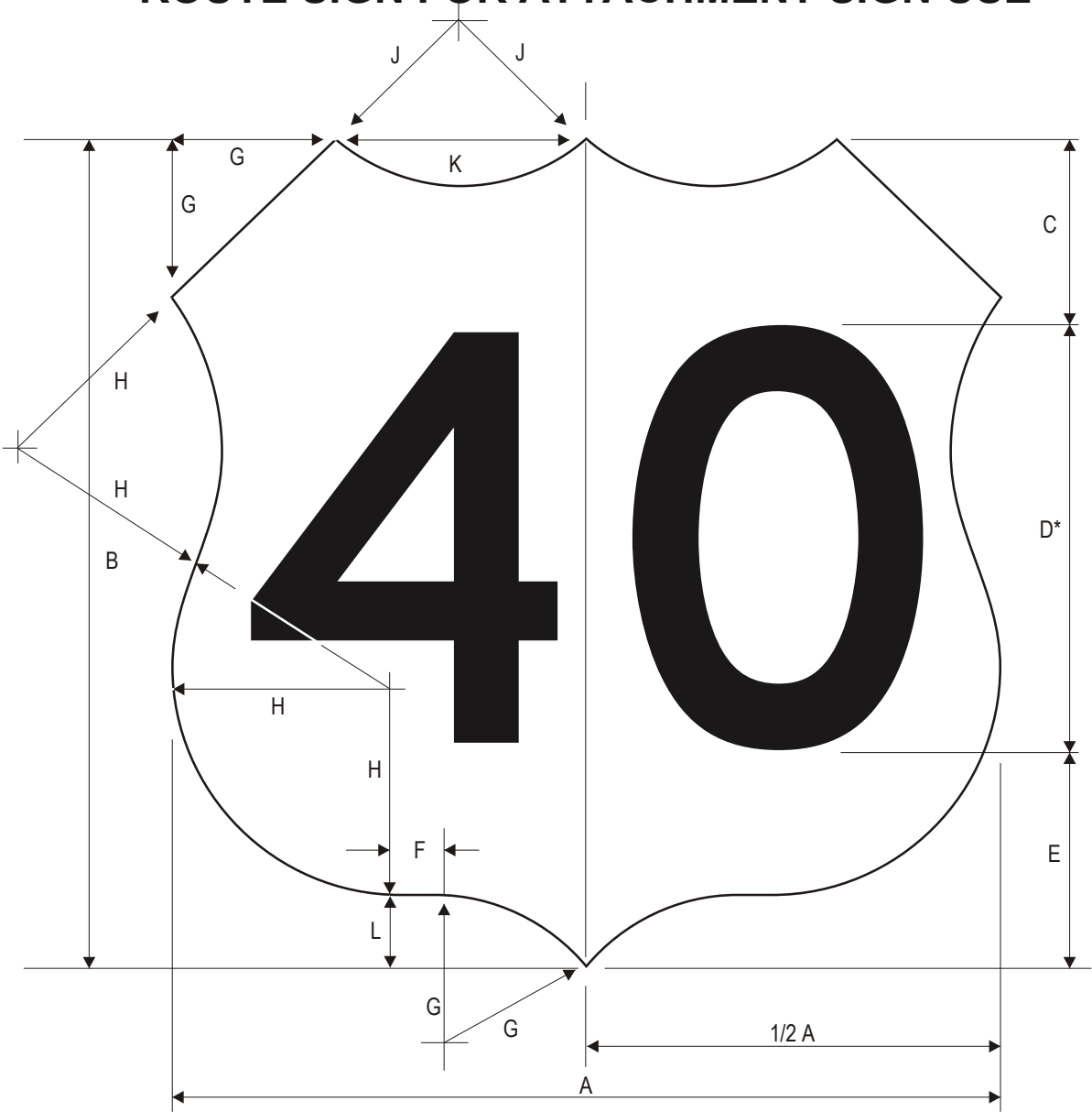
M1-4 U.S. Route Marker (Attachment)
