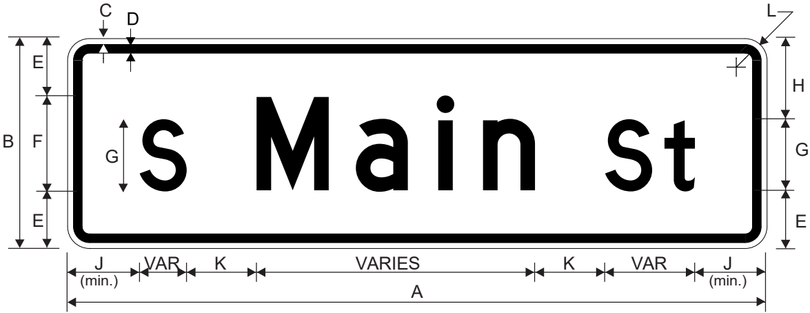
D3-1 Street Name (1 line)
